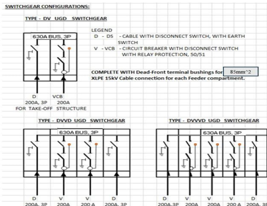
Figure 4. Switchgear Configurations
