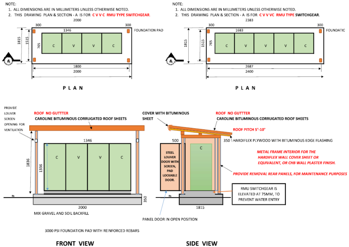
Figure 5. Plan and Sections views of the Padmount UGD Switchgear Housing
