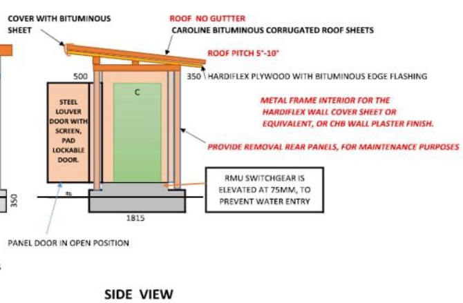
Figure 5. Plan and Sections views of the Padmount UGD Switchgear Housing
