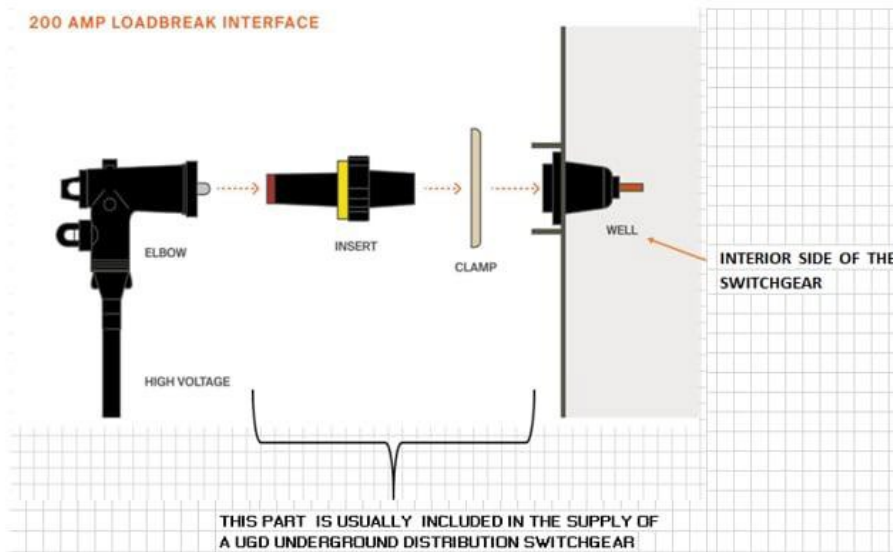
Figure 6. PRIMARY MV, SWITCHGEAR TERMINAL BUSHING
