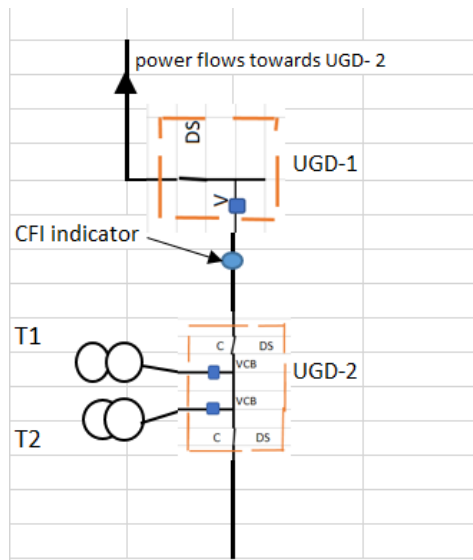
Diagram 1 , shows VCB of UGD-1 in normal condition on the Feeder circuit.
