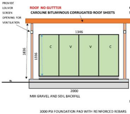
Figure 5. Plan and Sections views of the Padmount UGD Switchgear Housing
