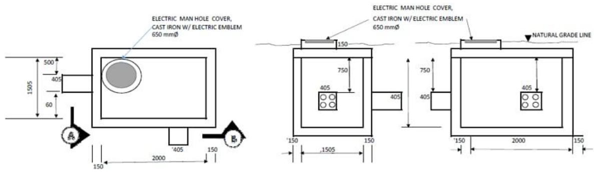
15KV MANHOLE, CORNER RUN TYPE
