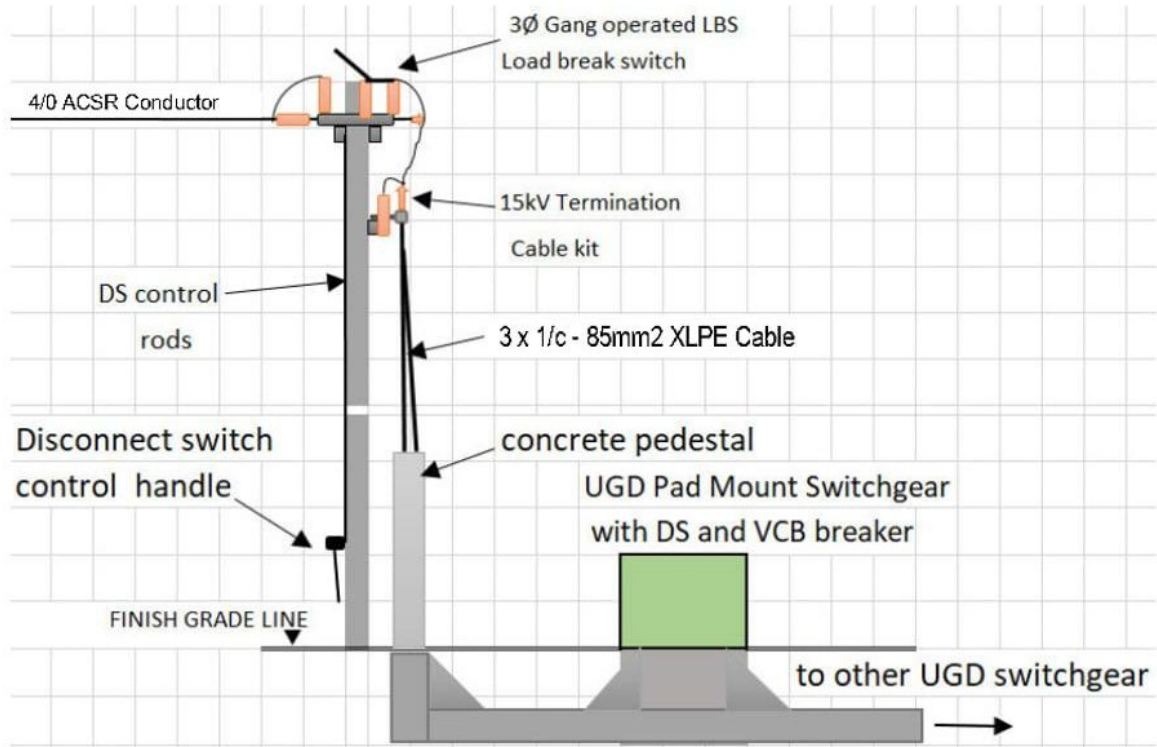
Figure 7. Take-off Structure
