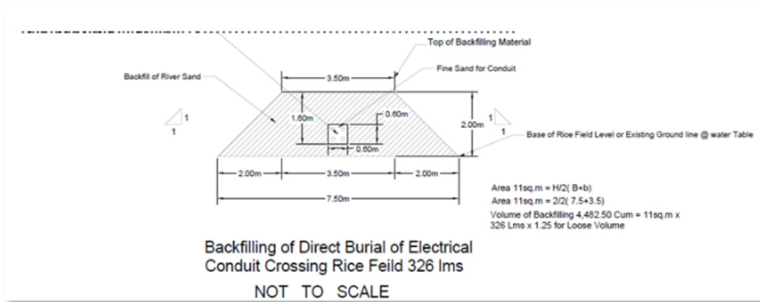
Figure 15. Underground Duct Bank Design for Crossing Rice Fields in Phase 4
