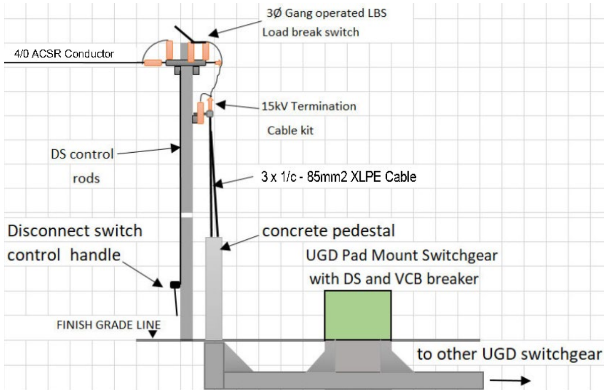
Figure 7. Take-off Structure
