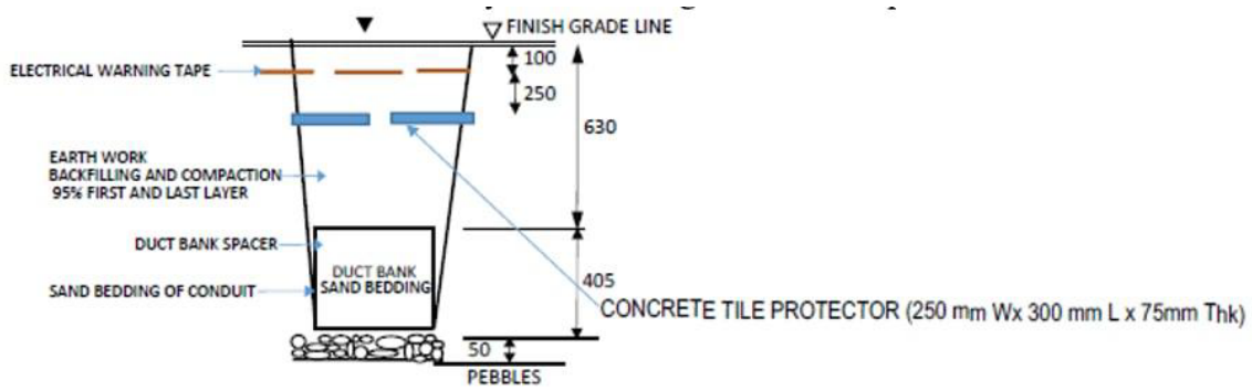
DETAILS OF DUCT BANK EXCAVATION N T S
