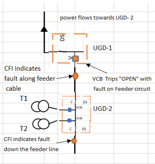
Diagram 2 , shows VCB of UGD-1 Trips "OPEN" to isolate the fault on the Feeder circuit.
